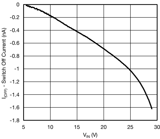
Fig. 8 - Shutdown Current vs. Input Voltage
