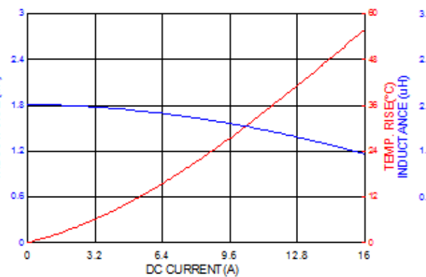
ASPIAIG-F5030-1R8
