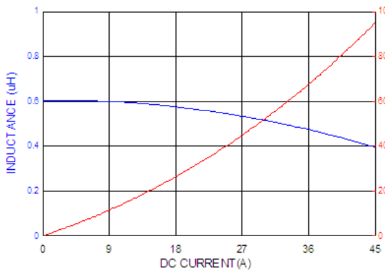
ASPIAIG-F7030-R60
