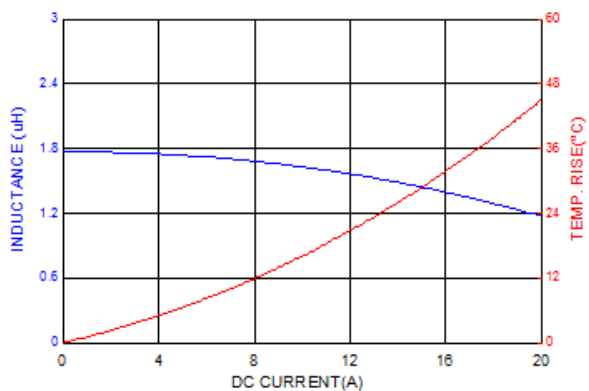
ASPIAIG-F6050-1R8
