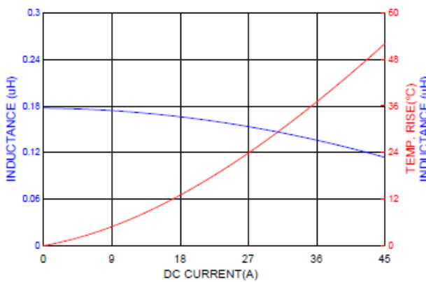
ASPIAIG-F6030-R18
