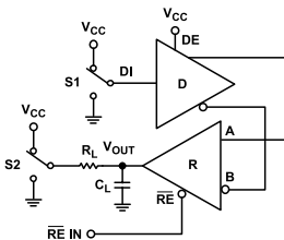
Figure 43. Receiver Enable/Disable from Shutdown
